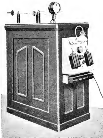
FIG. 2.—Alternating current high-tension rectifier. (Siemens.)
